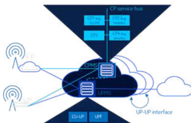
Figure 10: RAN Core Convergence
