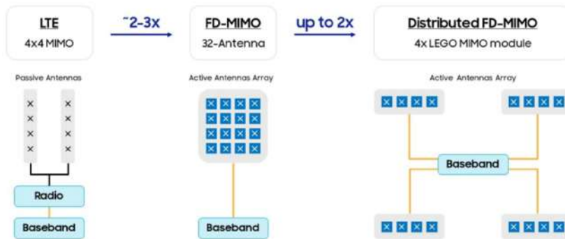
Figure 9: comparison of LTE, FD-MIMO and D-FD-MIMO deployment scenarios 97
