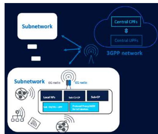
Figure 12: 6G sub-network interconnection architecture
