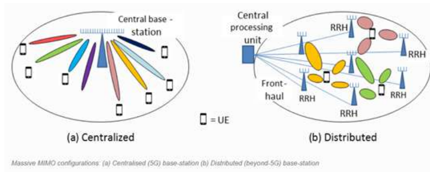
Figure 8: Massive MIMO configuration (a) Centralized (5G) Base Station (b) Distributed (beyond-5G) base-station 96
