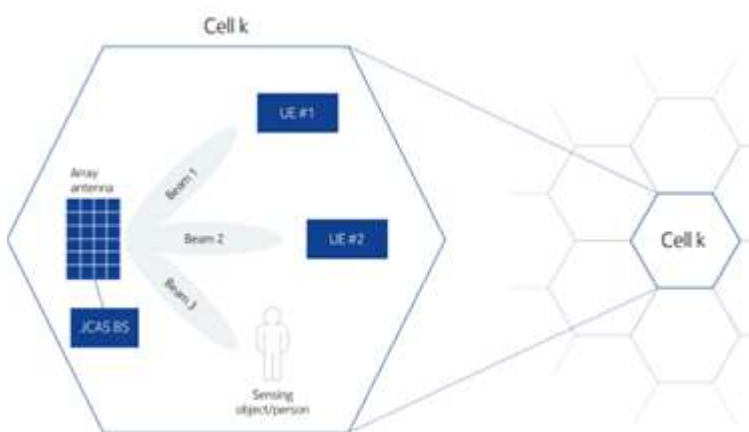
Figure 6: Basic joint communication and sensing (JCAS) system
