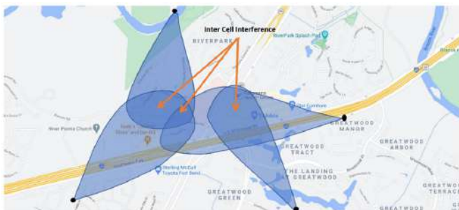
Figure 7: Inter-cell interference effects
