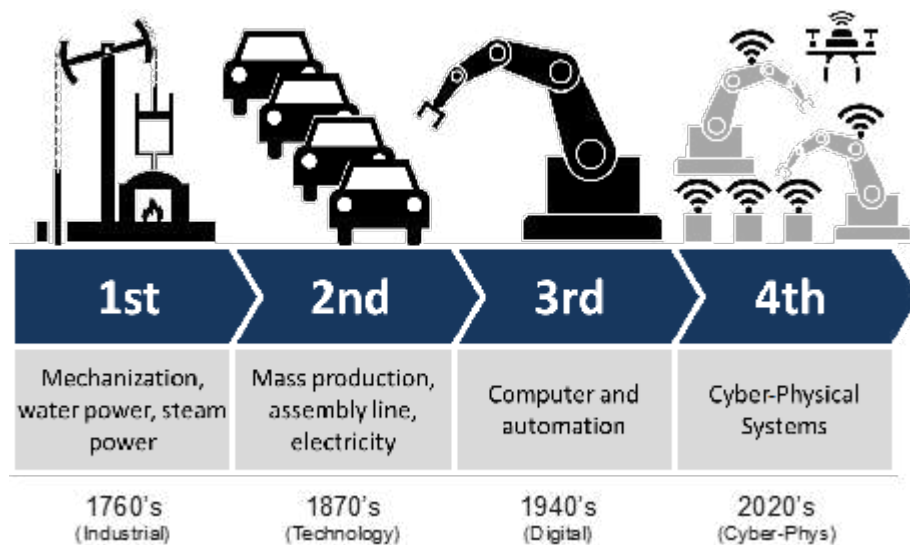
Figure 15: Industrial Revolutions
